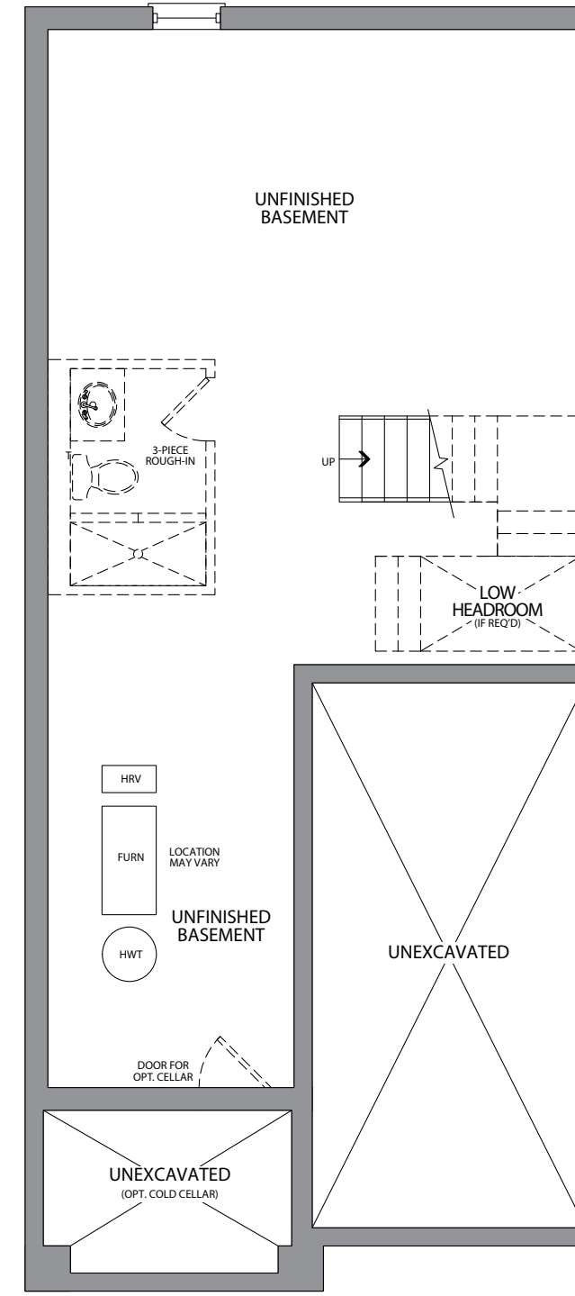
BASEMENT ELEV. A1/A2
