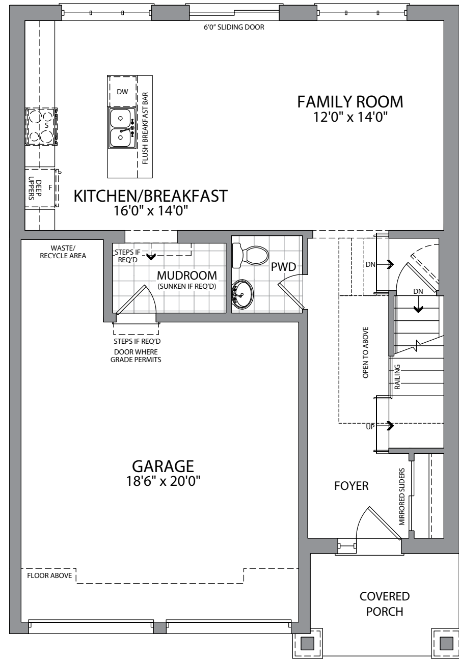
MAIN FLOOR ELEV. A
