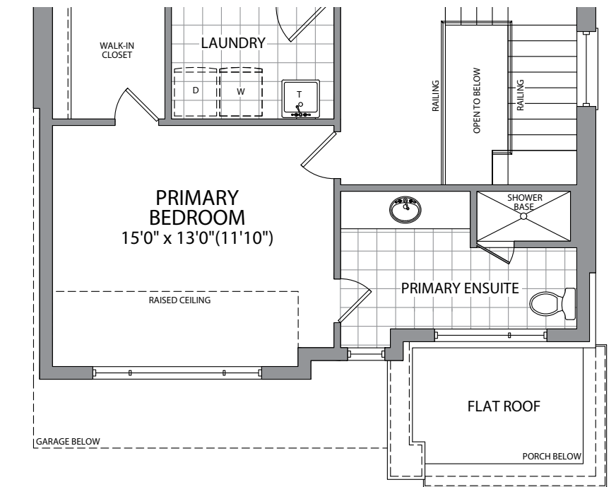
UPPER FLOOR ELEV. B
