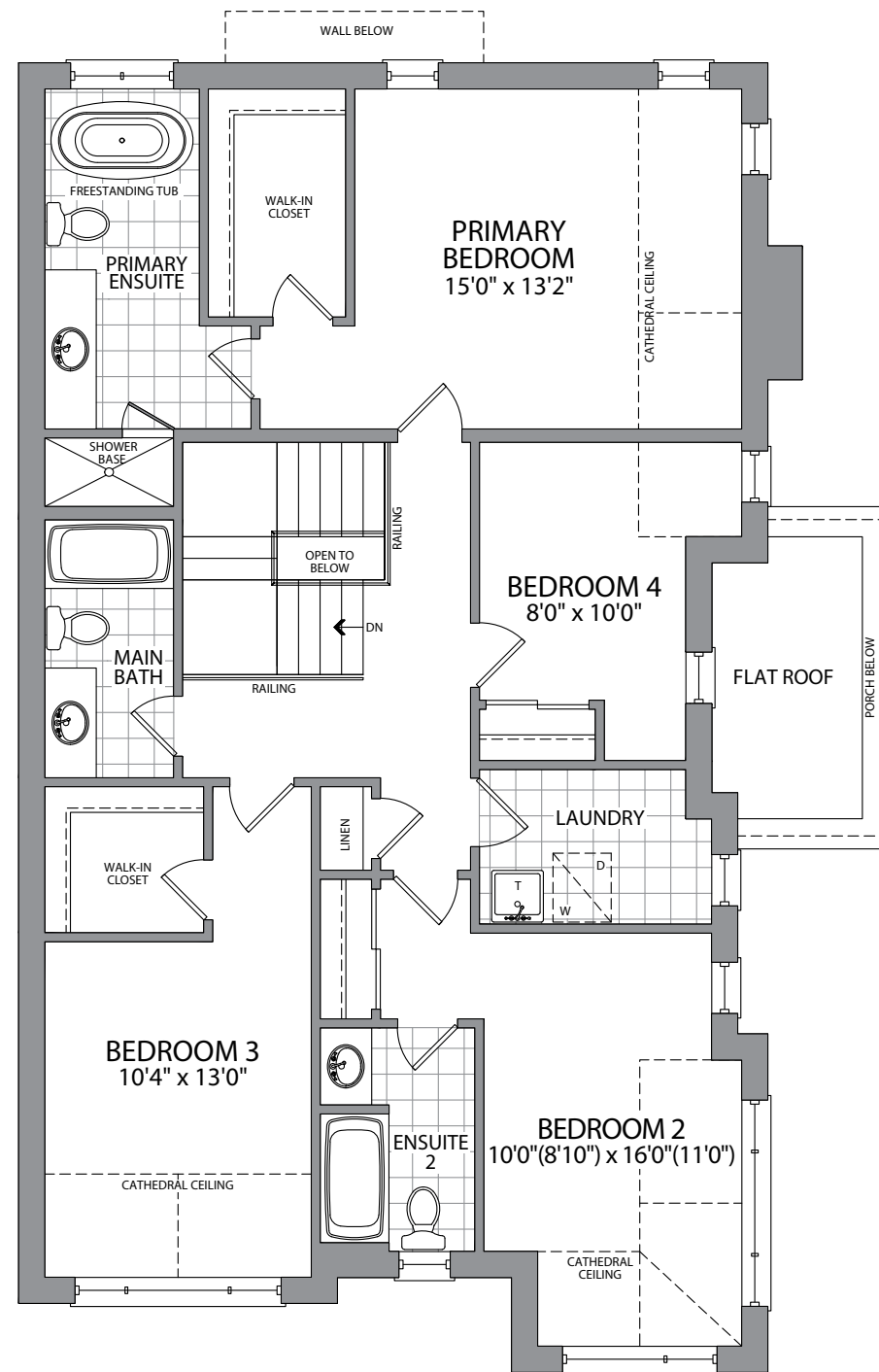
UPPER FLOOR ELEV. A
